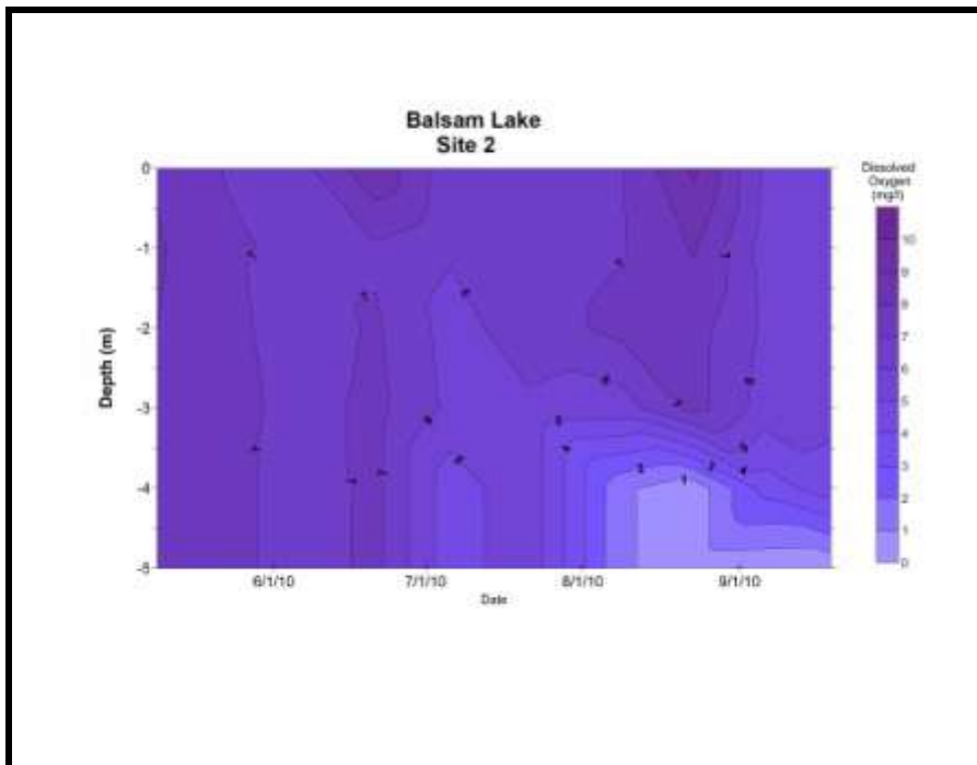
Figure 37 2010 S2 Dissolved Oxygen Isopleths
